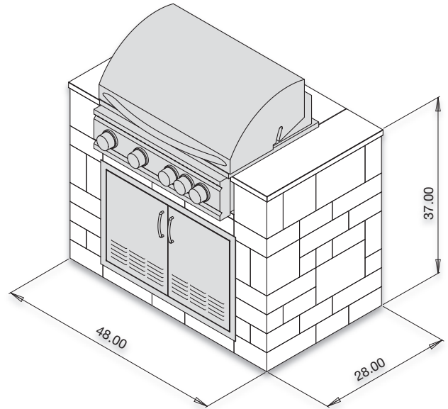
32" Sizzler Grill Cabinet
