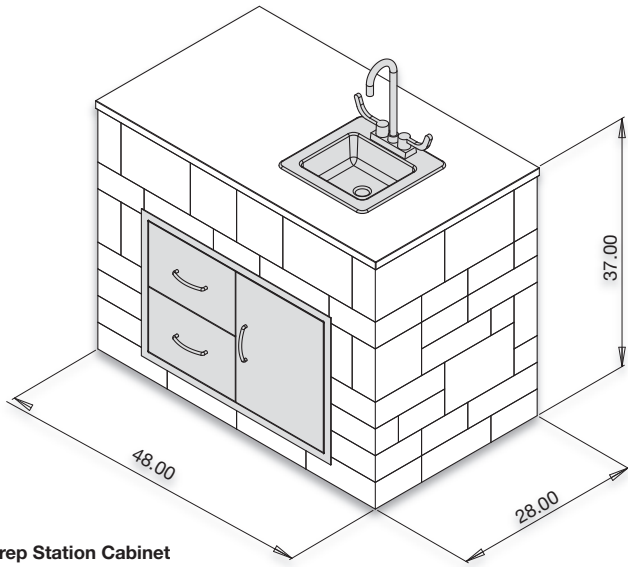
Prep Station Cabinet Optional sink
